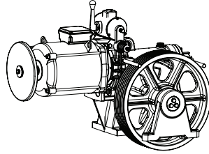
volpi VF3-9,0 kW 1,0 M-1125 KG
