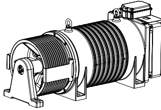
VOLPI VOLPI MRL 2-8 1,0 M-3500 KG
